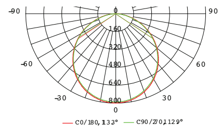
Oak Down Light 12W, 6500K
