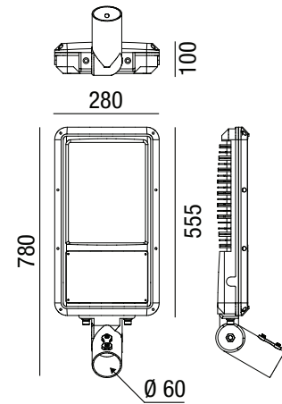
Dimension Diagram
